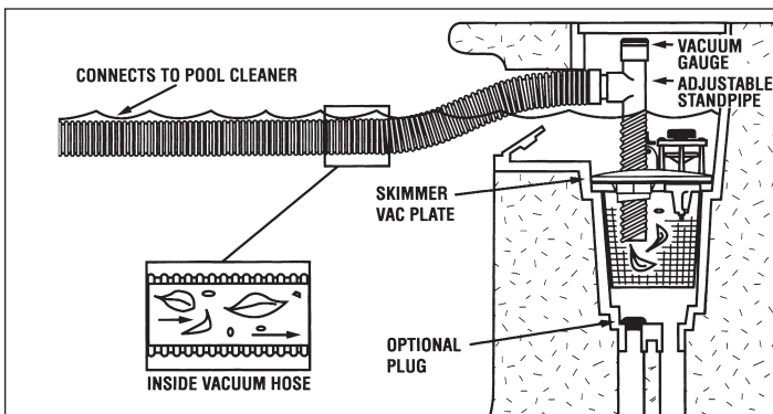
Hayward Skimmer Vacuum Plate
